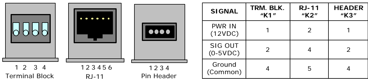
Figure 3.4 – Sensor Connector Signals – Sensor Head Side
