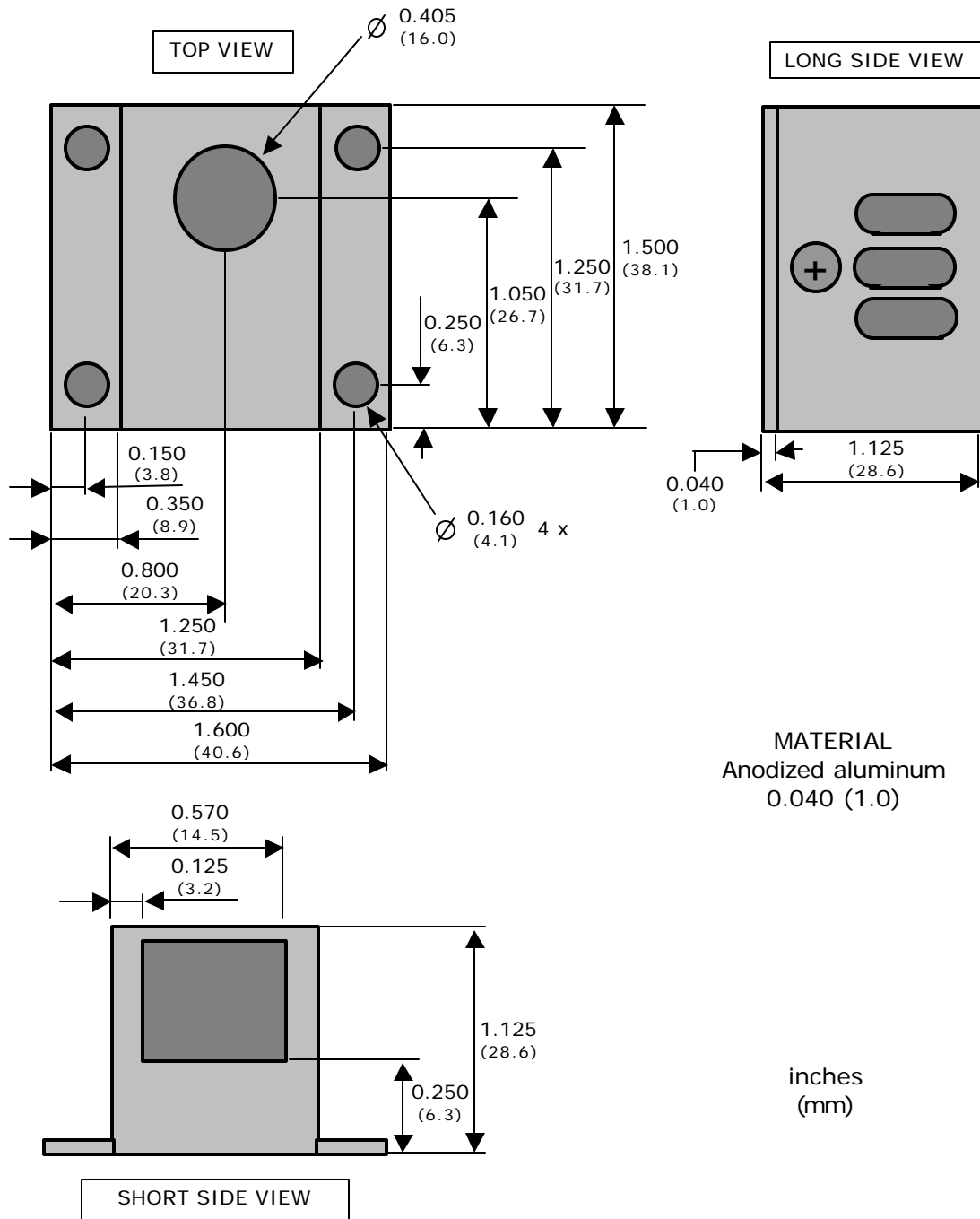
FIGURE. 4.2 – Sensor Head Dimensions
