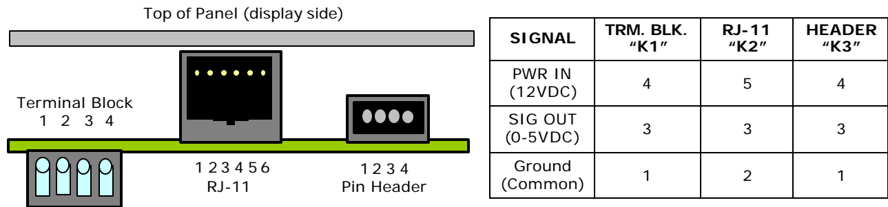
Figure 3.4 – Sensor Connector Signals – Sensor Head Side
