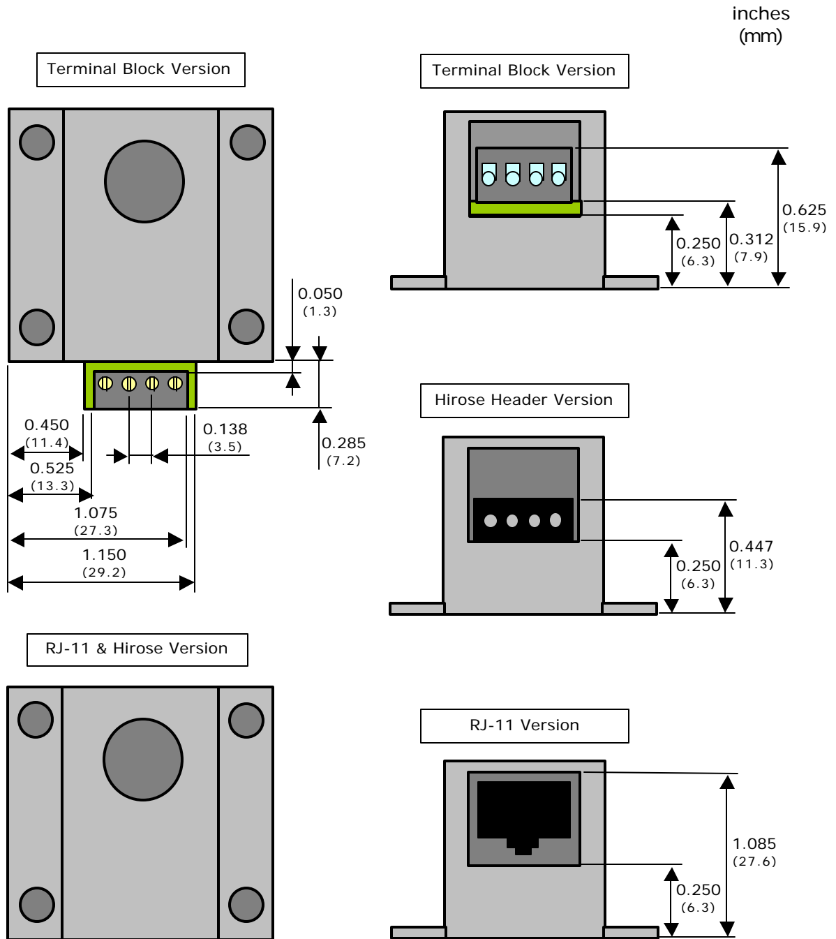
FIGURE. 4.3 – Sensor Head Connector Dimensions
