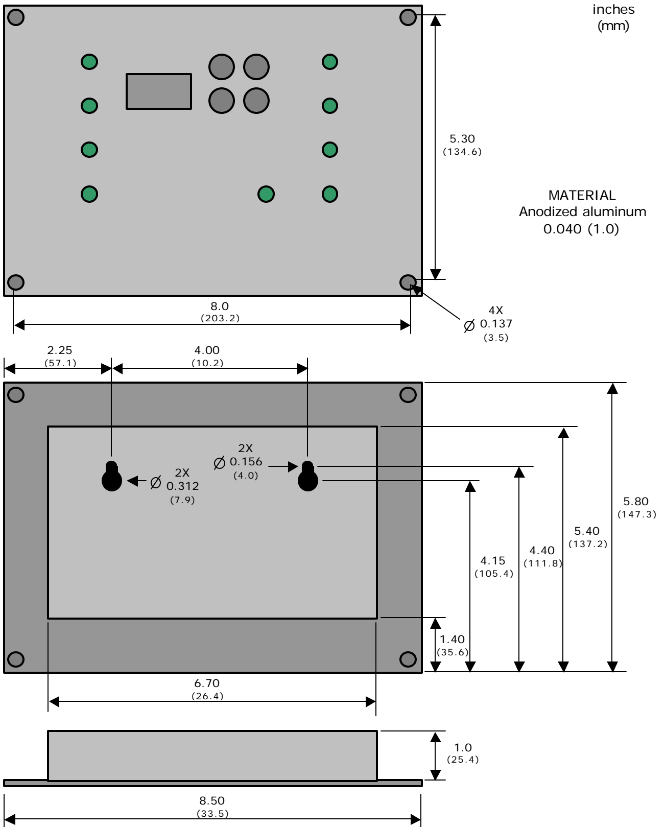
FIGURE. 4.1 – Panel Dimensions
